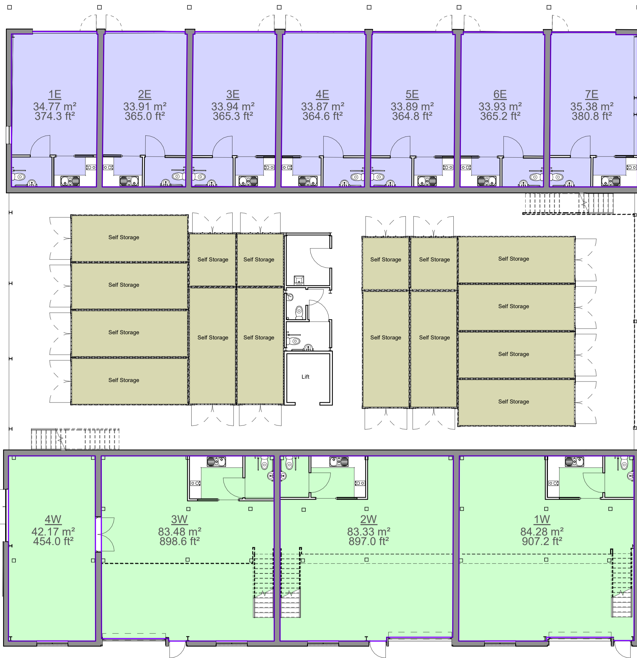
① Ground Level 1 : 100
